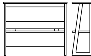
BBF97 Bookcase 36" wd x 12" dp x 30" hi
