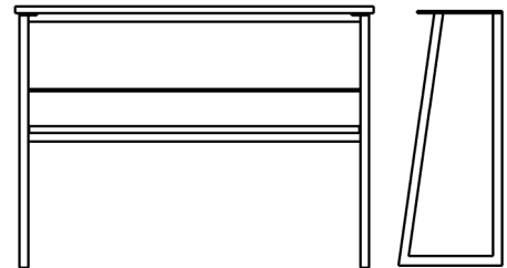
BBF097-500 ITrek II Bookcase 41-1/4" wd x 12" dp x 30" hi
