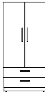
3279 Pulse Wardrobe 36" lg x 24" dp x 72" hi
